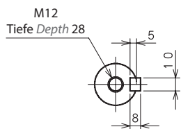
Genutete Welle Keved shaft
