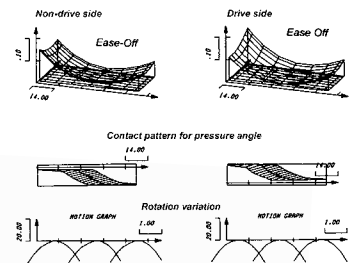
Optimized Gleason gearing for highest speeds
