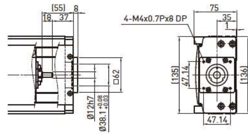
Motor Adaptor Flange F6
